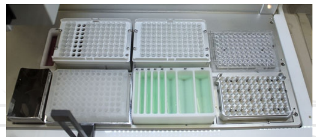
VERSA Gene 10 Deck Layout
